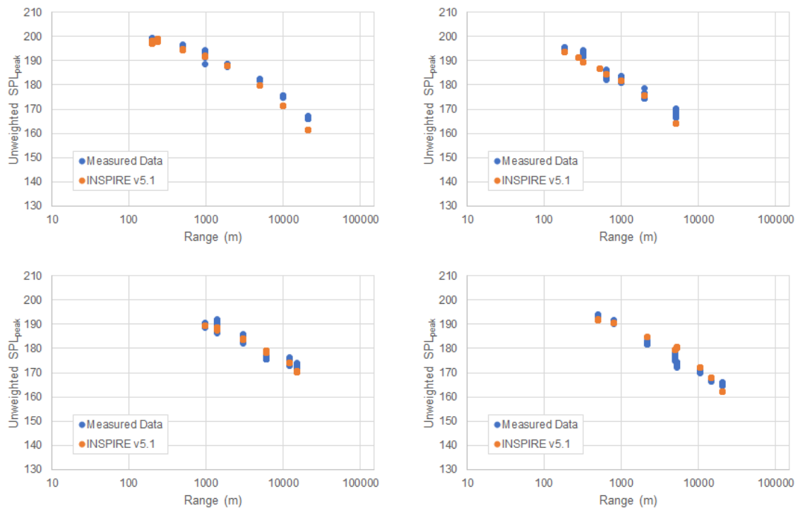
Figure 4-1 Comparison between example unweighted SPL_{peak} measured data (blue points) and modelled data using INSPIRE version 5.1 (orange points)
