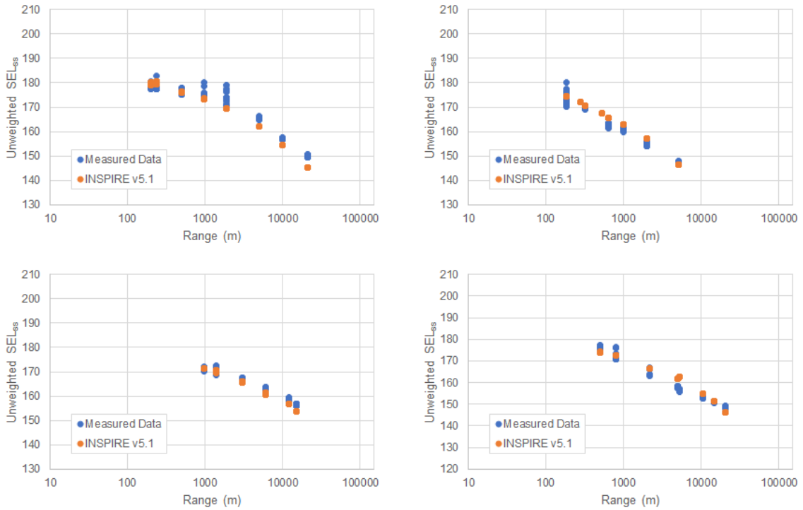
Figure 4-2 Comparison between example unweighted SEL_{ss} measured data (blue points) and modelled data using INSPIRE version 5.1 (orange points)
